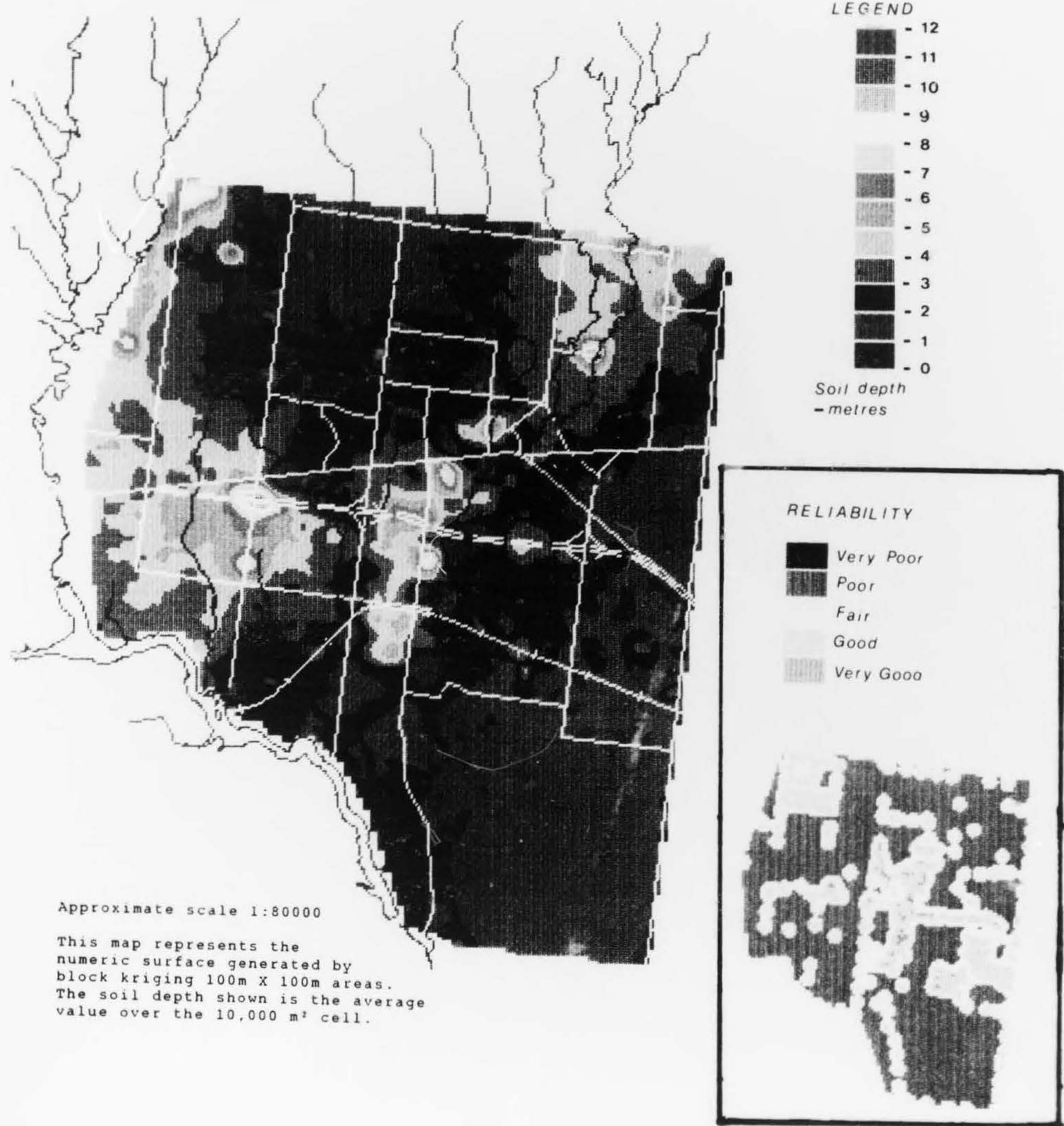
Figure 5. Soil depth map.
