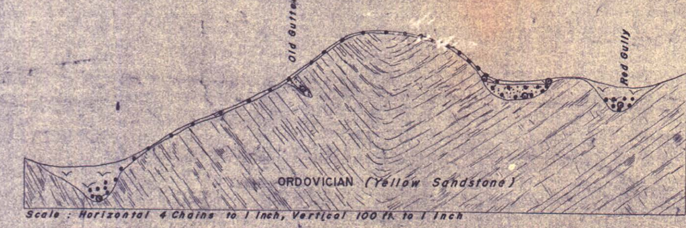
SECTION THROUGH COLLINS CLAIM 2 MILE CREEK
