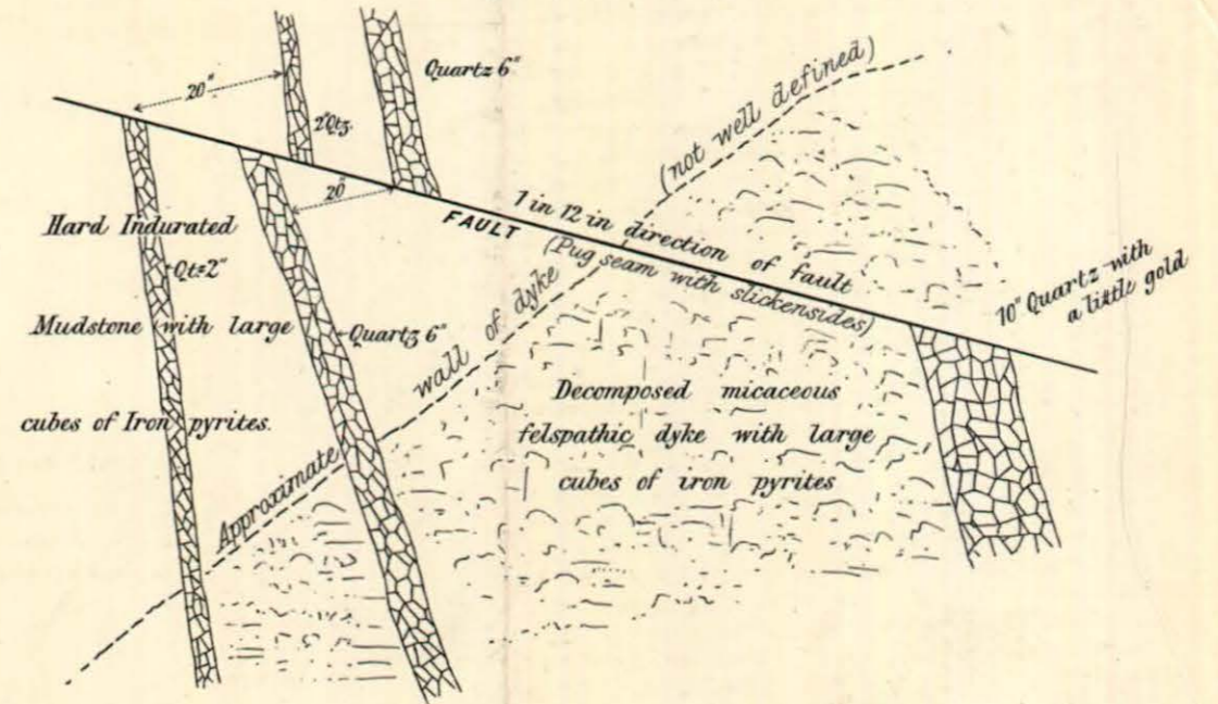
FIG. I Sketch Section M c LAREN'S CLAIM (Looking South) Scale, about 2 Feet to 1 Inch.
