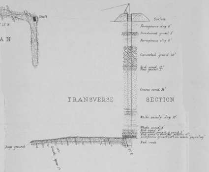
UNDERGROUND WORKINGS OF HOOPER AND WEBSTER Scale of Feet
