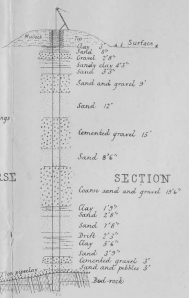
UNDERGROUND WORKINGS OF LETHLEAN AND PARTY Scale of Feet
