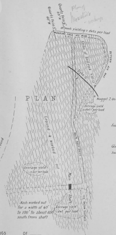
UNDERGROUND WORKINGS OF LETHLEAN AND PARTY Scale of Feet
