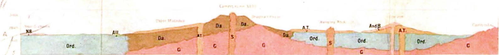
SECTION A B FROM S TO N THROUGH MT MACEDON
